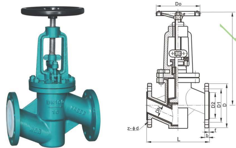
衬氟截止阀 (J41F4)
